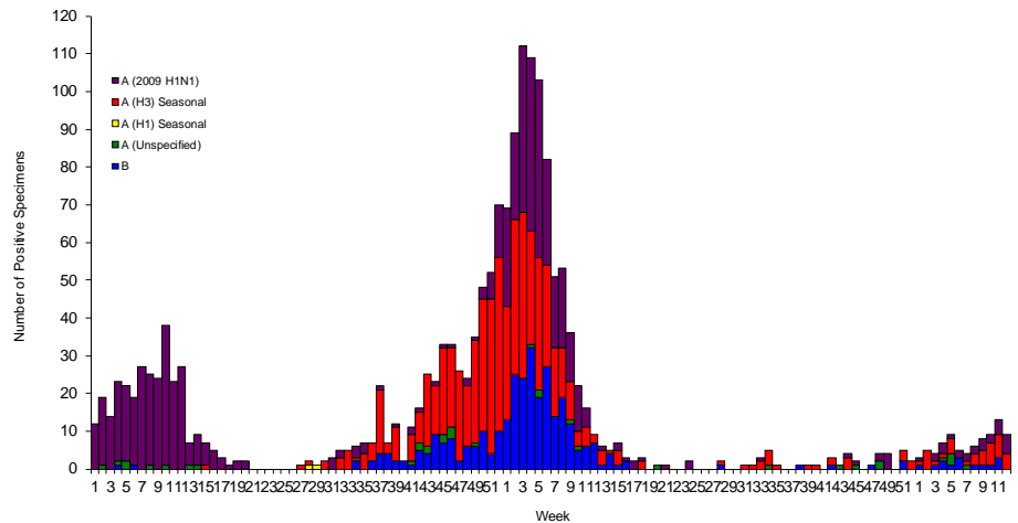
Figure 13: Number of Influenza-Positive Specimens Tested by the Florida Bureau of Laboratories (BOL) by Subtype by Lab Event Date* Week 1, 2010 to Week 12, 2012 as Reported in Merlin by 11:30 a.m. March 28, 2012
