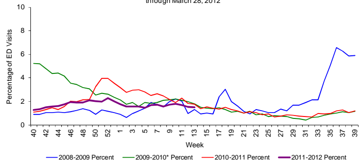
Figure 10: Percentage of Influenza-Like Illness from Emergency Department (ED) Chief Complaints, RDSTF Region 5 ESSENCE Participating Hospitals (N=49), Week 40, 2008 through March 28, 2012
