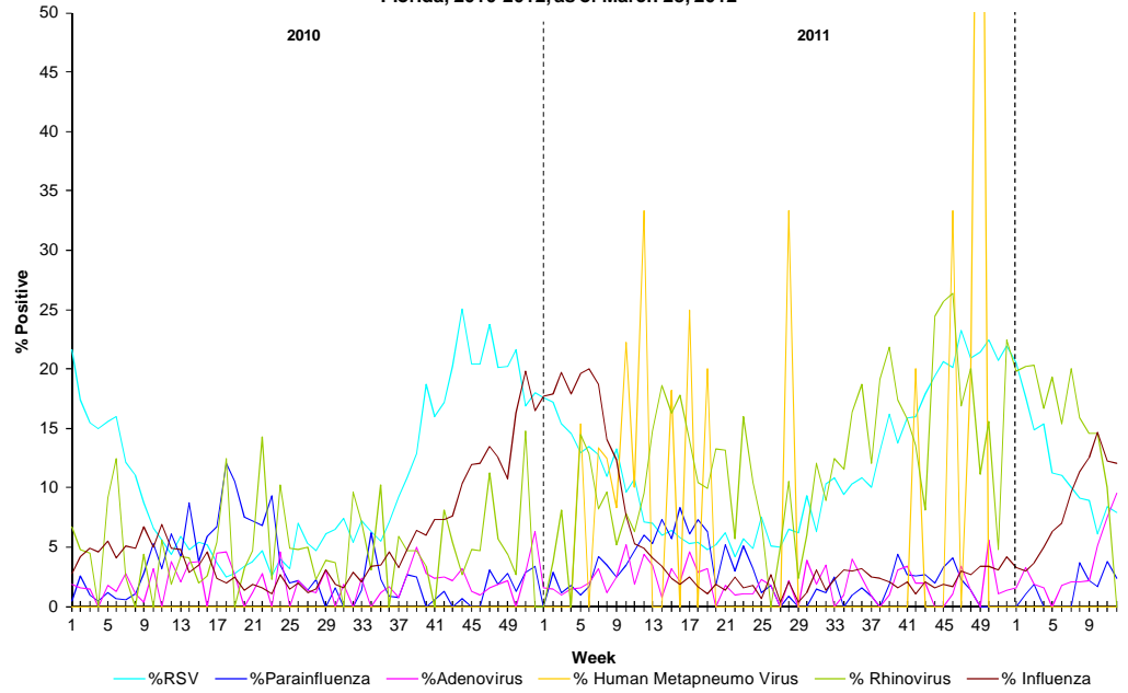
Figure 28: Percentage of Positive Respiratory Virus Tests as Collected by NREVSS, Florida, 2010-2012, as of March 28, 2012
