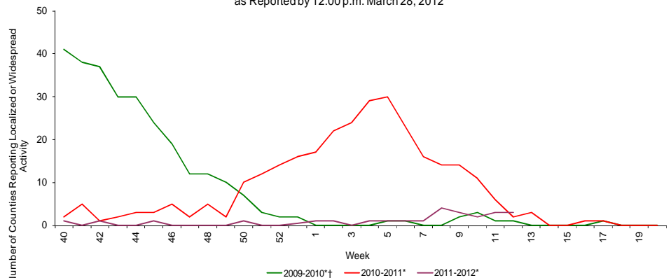
FIGURE 15: Number of Counties Reporting Moderate (Localized) or Widespread Activity, 2009-2010 (Weeks 40-20), 2010-2011 (Weeks 40-20), and 2011-2012 (Weeks 40-12) as Reported by 12:00 p.m. March 28, 2012
