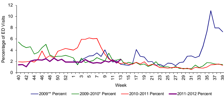
Figure 9: Percentage of Influenza-Like Illness from Emergency Department (ED) Chief Complaints, RDSTF Region 4 ESSENCE Participating Hospitals (N=31), Week 40, 2008 through March 28, 2012
