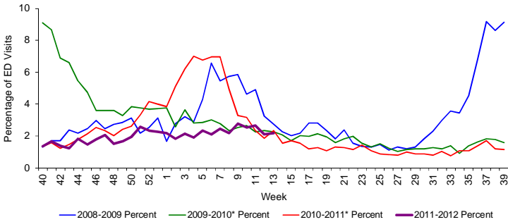
Figure 6: Percentage of Influenza-Like Illness from Emergency Department (ED) Chief Complaints, RDSTF Region 1 ESSENCE Participating Hospitals (N=5), Week 40, 2008 through March 28, 2012
