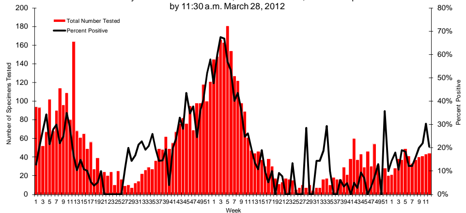
Figure 14: Number of Specimens Tested by Florida Bureau of Laboratories (BOL) and Percent Positive for Influenza by Lab Event Date* Week 1, 2010 to Week 12, 2012 as Reported in Merlin by 11:30 a.m. March 28, 2012
