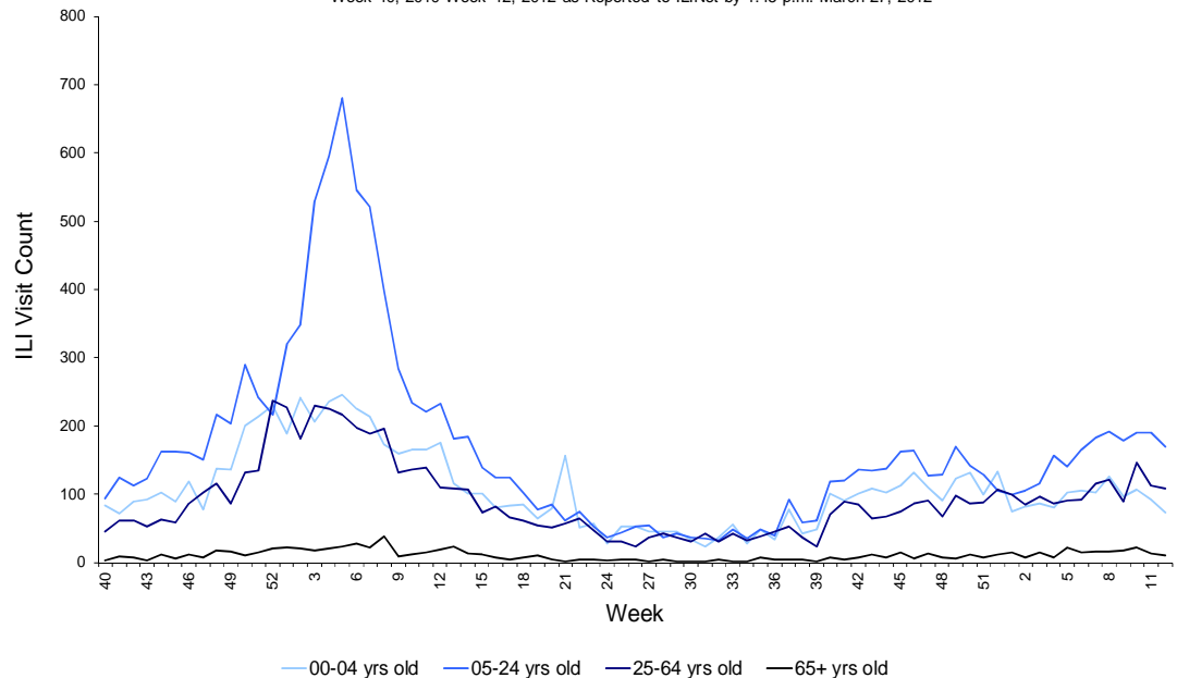
FIGURE 2: Influenza-like Illness (ILI) Visit Counts Reported by ILINet Sentinel Providers Statewide by Age Group Week 40, 2010-Week 12, 2012 as Reported to ILINet by 1:45 p.m. March 27, 2012
