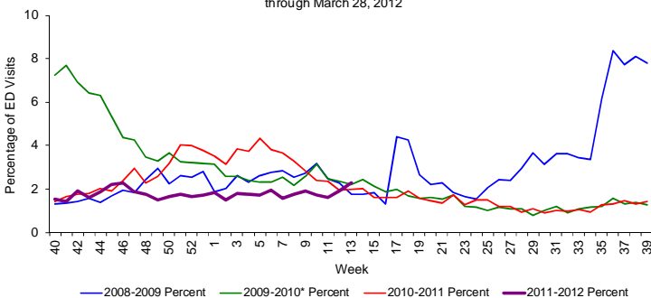
Figure 11: Percentage of Influenza-Like Illness from Emergency Department (ED) Chief Complaints, RDSTF Region 6 ESSENCE Participating Hospitals (N=15), Week 40, 2008 through March 28, 2012
