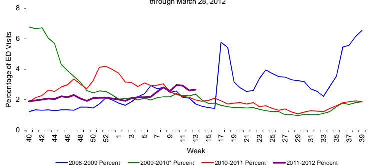
Figure 12: Percentage of Influenza-Like Illness from Emergency Department (ED) Chief Complaints, RDSTF Region 7 ESSENCE Participating Hospitals (N=48), Week 40, 2008 through March 28, 2012
