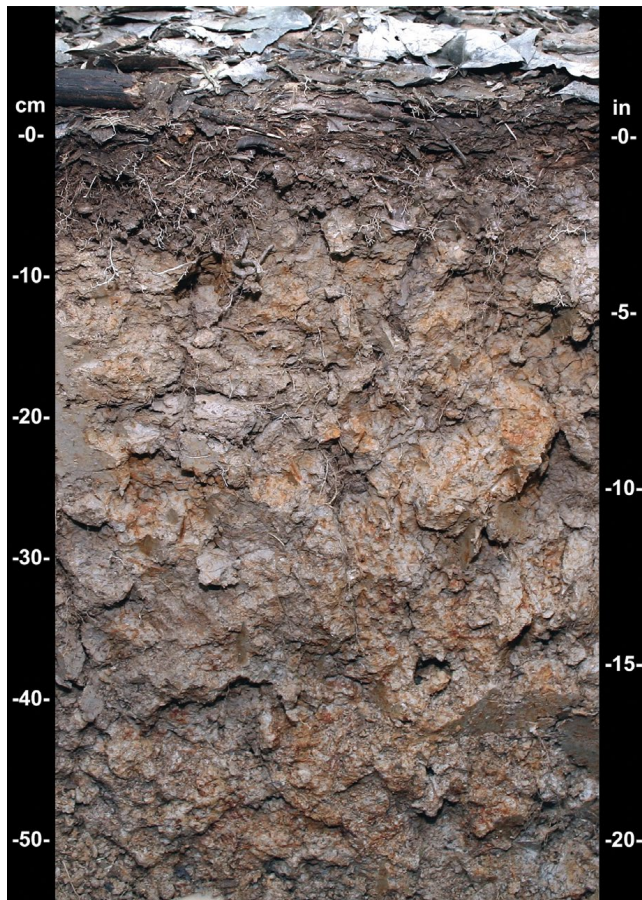
Figure 29.—Indicator F3 (Depleted Matrix). This soil has value of 4 or more and chroma of 2 or less and redox concentrations starting at a depth of 8 cm. Since the depleted matrix starts at a depth of \leq 15 cm from the soil surface, the minimum thickness requirement is only 5 cm.
